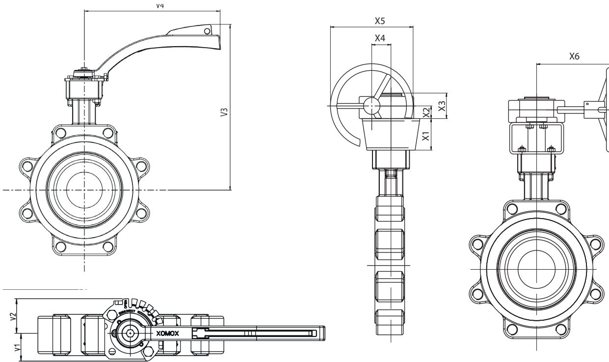
Valves with Latching Lever or Worm Gear DN 80 up to 600 / NPS 3" up to 24"
