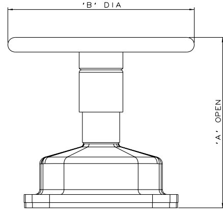
DN65 to DN80 only 2.5" - 3.0"
