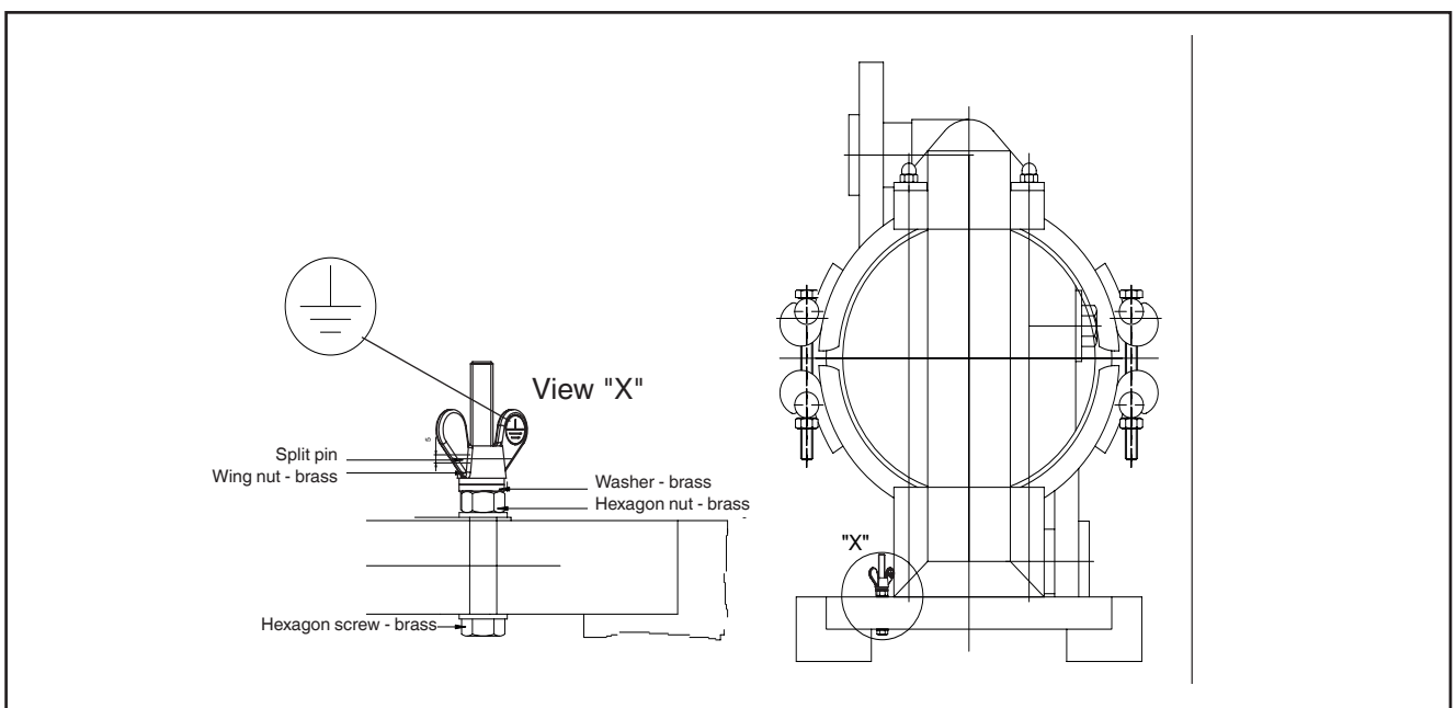
Fig. 5: Earthing screw
